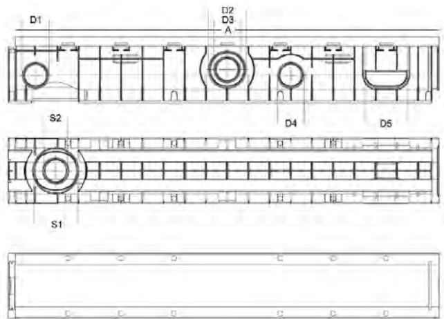
SABDRAIN 706
