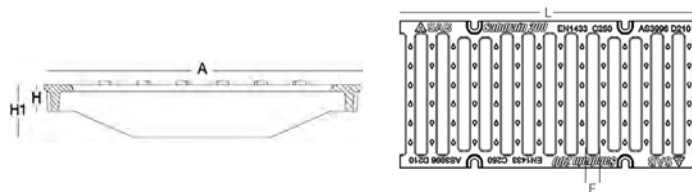
SABDRAIN 706 - GRATE
