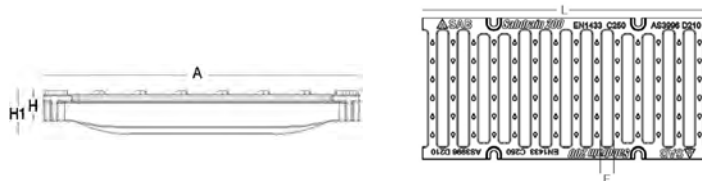
SABDRAIN 705 - GRATE
