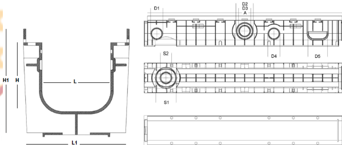
SABDRAIN 501
