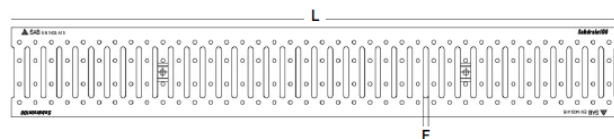
SABDRAIN 501 - GRATE
